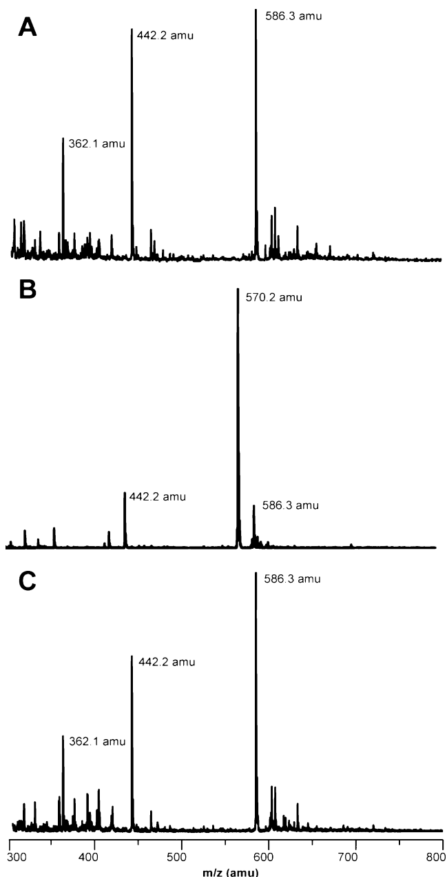
FIGURE 5: ESI mass spectra of wild-type and ColD H188K reactions. The spectrum of the reaction without the addition of ColD is given in Panel A and shows the buildup of GDP-4-keto-6-deoxymannose at 586.3 amu. Additional peaks at 442.2 and 362.1 amu result from the partial breakdown of this compound into GDP and GMP, respectively. The reactions with wild-type ColD given in Panel B show conversion of the 586.3 amu peak into a new peak at 570.2 amu, which is the appropriate mass of the ColD reaction product, GDP-4-keto-3,6-dideoxymannose. The reaction with ColD H188K shown in Panel C indicates a buildup of GDP-4-keto-6-deoxymannose and breakdown compounds.
