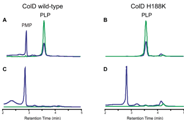
FIGURE 4: Formation of PMP by ColD. The elution was monitored at 320 nm (blue traces) and 395 nm (green traces). The resting form of wild-type ColD contains both PMP and PLP as indicated in Panel A. The resting form of ColD H188K contains only PLP (Panel B). When the enzyme in excess is incubated with PLP, near complete conversion of the PLP to PMP is observed for both the wild-type and mutant proteins as indicated in Panels C and D. The formation of PMP by the mutant protein can either be a result of true aminotransferase activity or a breakdown of the geminal diamine intermediate as a consequence of boiling.
