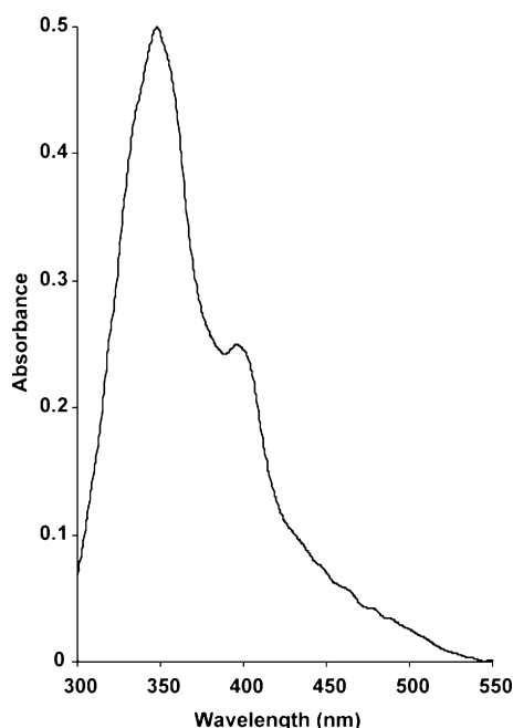
FIGURE 2: Single-crystal UV/visible absorption spectrum. The absorption spectrum from a ColD H188K single crystal shows two major peaks at 345 and 400 nm.
