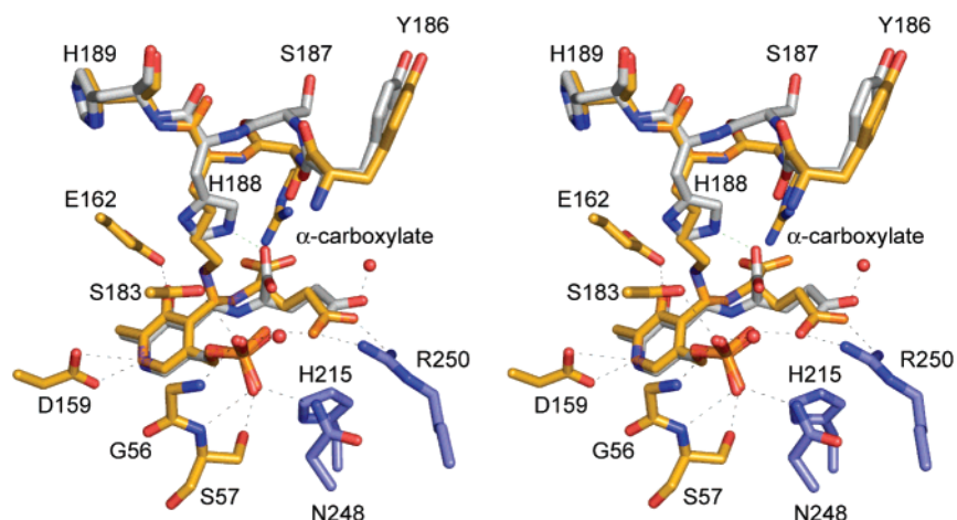
FIGURE 3: Superposition of the geminal diamine intermediate onto the ketimine intermediate. The model corresponding to ColD H188K is displayed in gold and slate bonds for Subunits 1 and 2, respectively. The positions of His 188 and the ketimine intermediate in the wild-type ColD model are highlighted in white bonds. Dashed lines indicate interactions within 3.2 Å of respective atoms.
