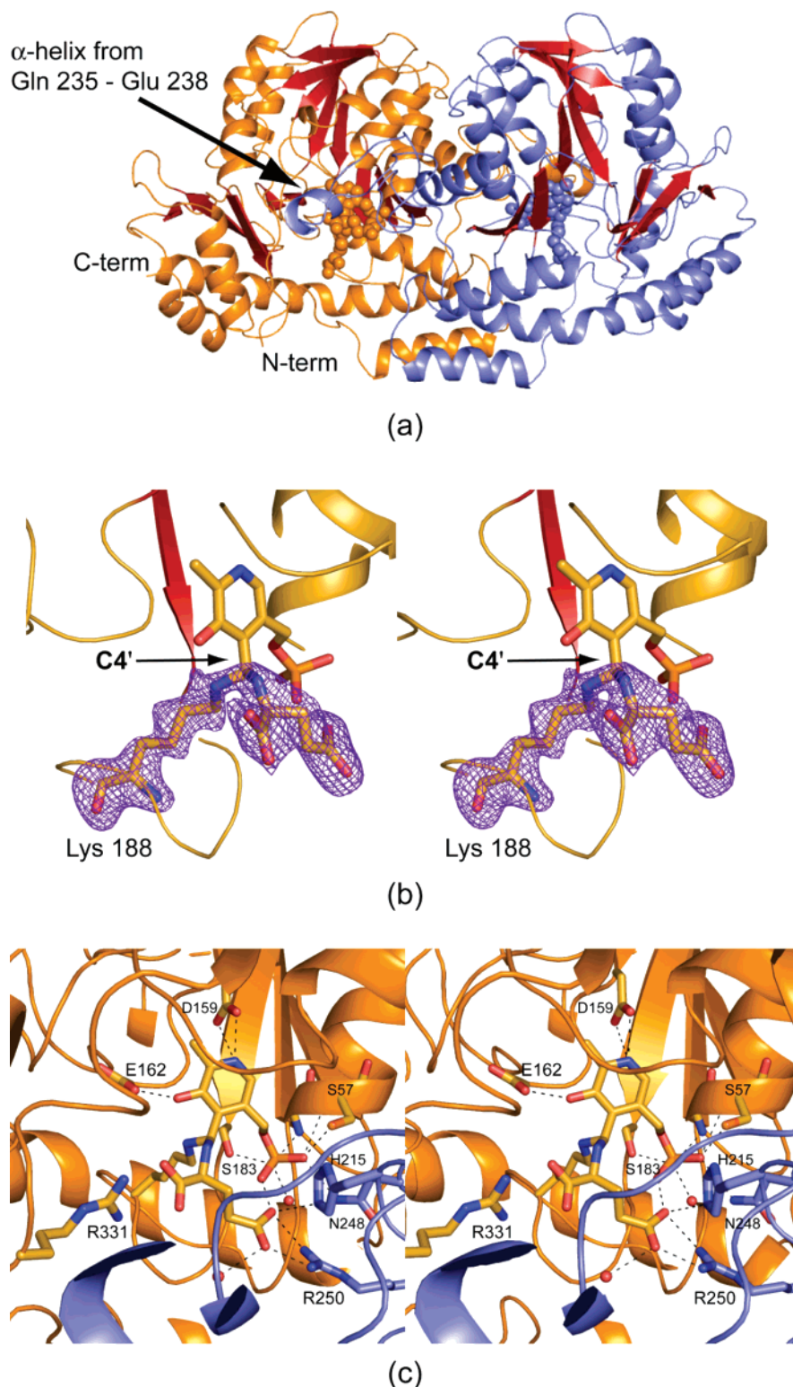
FIGURE 1: The structure of H188K CoID. (a) A ribbon representation of the dimeric protein with Subunits 1 and 2 color coded in gold and slate, respectively. The positions of the active sites are indicated by the space-filling representations for the geminal diamine intermediates. (b) Electron density corresponding to this intermediate in Subunit 1. The map was calculated with coefficients of the form (F_o - F_c) , where F_o was the native structure factor amplitude and F_c was the calculated structure factor amplitude. Atoms corresponding to the intermediate and Lys 188 were excluded from the coordinate file during the least-squares refinement. The map was contoured at \sim 3\sigma . (c) A close-up view of the active site for Subunit 1. Those interactions between the intermediate and the protein, within 3.2 Å, are indicated by the dashed lines. Figures 1 and 3 were prepared with the software package PyMOL (28).
